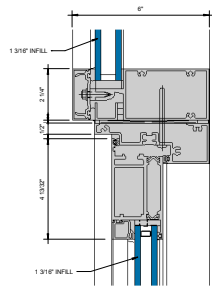
⑤ 2000T TERRACE DOOR HEADER @ HORIZONTAL 6" = 1'-0"
