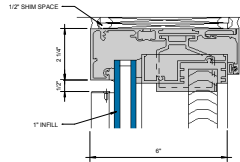
HEAD STANDARD RECEPTOR W/ ② OPTIONAL BLIND POCKET 6" x 1-1/2"
