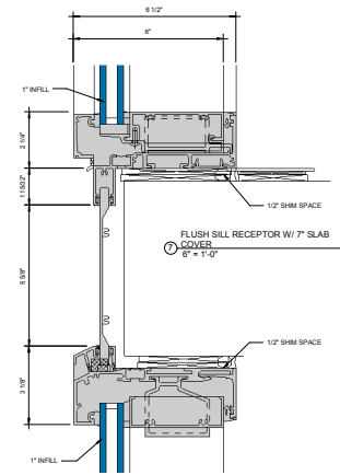
FLUSH HEAD RECEPTOR W/ OPTIONAL ① WEDGE GASKET ② 6" x 1"-0"
