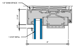
① HEAD STANDARD RECEPTOR 6" = 1'-0"
