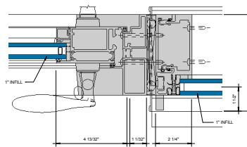
⑥ ALTERNATE SSG DOOR JAMB @ LOCK STILE 6" = 1'-0"
