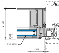
GLASSvent UT JAMB (RH) AT VERTICAL POCCOS Ø = 1-0"
