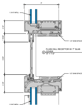
⑥ FLUSH HEAD RECEPTOR W/ REINFORCEMENT 6" x 1'-0"
