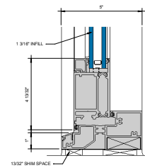
⑦ 2000T TERRACE DOOR SILL 6" = 1'-0"
