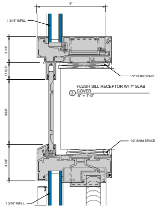
③ FLUSH SILL RECEPTOR W/ 7" SLAB COVER 6" x 1'-0"
