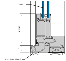
① 2000T TERRACE DOOR SILL 6" = 1'-0"
