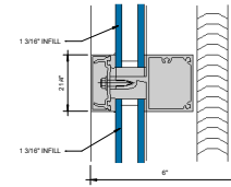
⑦ HORIZONTAL BLIND APPLICATION 6" = 1'-0"
