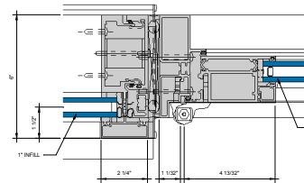
② DOOR JAMB @ HINGE STILE Ø = 1'-0"
