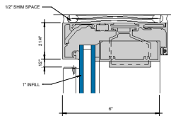
HEAD STANDARD RECEPTOR W/ ⑤ REINFORCEMENT 6" x 1-1/2"
