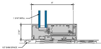
⑨ SILL STANDARD RECEPTOR W/ OPTIONAL STRAP ANCHOR 6" = 1'-0"
