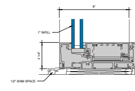
⑧ SILL STANDARD RECEPTOR 6" x 1-1/2"
