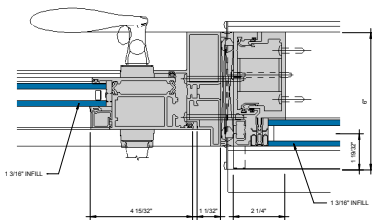
⑨ ALT. SSG DOOR JAMB @ LOCK STILE Ø = 1'-0"
