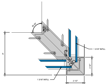
① 90° OUTSIDE CORNER G = 1'-0"
