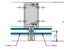
④ VERTICAL MULLION 6" = 1'-0"
