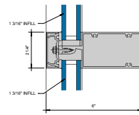
② HORIZONTAL 6" = 1'-0"
