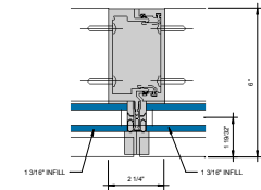
4 ALT. SSG VERTICAL MULLION 6" = 1'-0"
