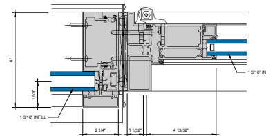
⑪ DOOR JAMB @ HINGE STILE 6" = 1'-0"
