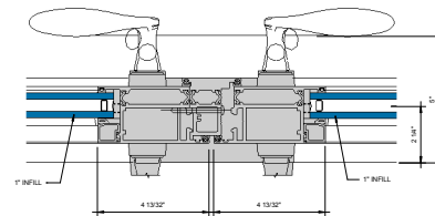
⑩ 2000T DOOR MEETING STILES Ø = 1'-0"
