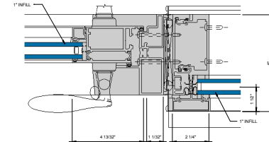
⑫ DOOR JAMB @ LOCK STILE 6" = 1'-0"
