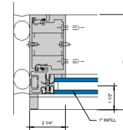
③ ALT. SSG JAMB 6" = 1'-0"
