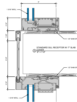
STANDARD HEAD RECEPTOR W/ ③ OPTIONAL STRAP ANCHOR 6" = 1'-0"
