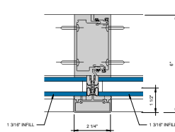
⑩ VERTICAL MULLION 6" = 1'-0"
