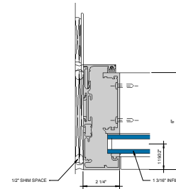
③ JAMB RECEPTOR AND STRAP ANCHOR h = 1'-0"
