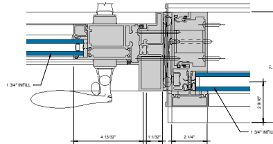
2 DOOR JAMB @ LOCK STILE 6" = 1'-0"
