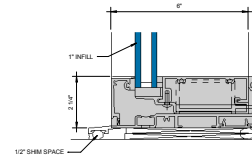
③ SILL W/ PUNCHED OPENING RECEPTOR 6" = 1'-0"
