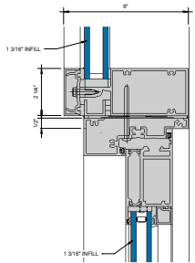
⑤ 2000T TERRACE DOOR HEADER @ HORIZONTAL 6" = 1'-0"
