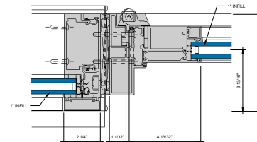
⑪ DOOR JAMB @ HINGE STILE 6" = 1'-0"
