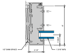
② JAMB RECEPTOR h = 1'-0"
