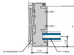
② JAMB RECEPTOR 6" = 1'-0"
