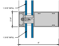
② HORIZONTAL 6" = 1'-0"
