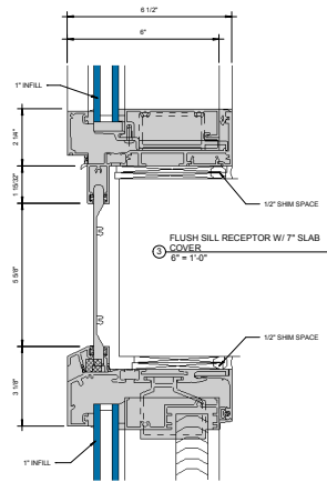
FLUSH HEAD RECEPTOR W/ OPTIONAL ① BLIND POCKET ② 6" x 1"-0"
