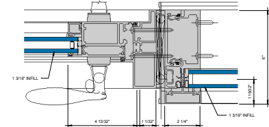
⑫ DOOR JAMB @ LOCK STILE 6" = 1'-0"
