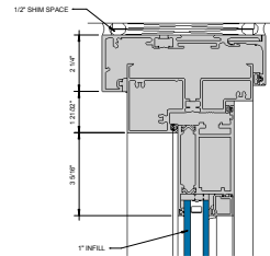
2000T TERRACE DOOR HEADER W/ PUNCHED OPENING RECEPTOR ⑥ 6" = 1'-0"
