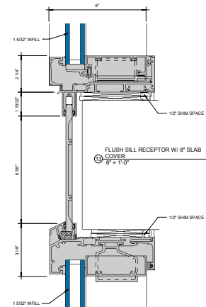
⑭ FLUSH HEAD RECEPTOR W/ OPTIONAL BLIND POCKET 6" = 1'-0"
