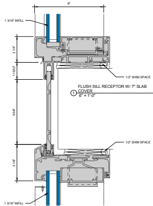
② FLUSH HEAD RECEPTOR 6" x 1'-0"
