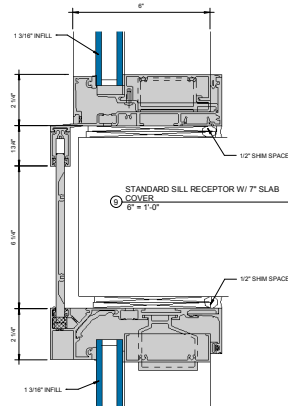
STANDARD HEAD RECEPTOR W/ ⑤ REINFORCEMENT 6" = 1'-0"
