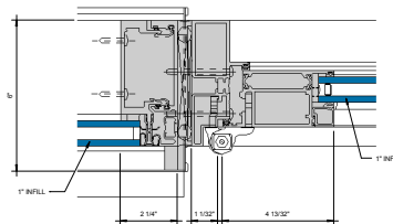
⑥ ALT. SSG DOOR JAMB @ HINGE STILE Ø = 1'-0"
