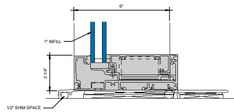
⑨ SILL STANDARD RECEPTOR W/ OPTIONAL STRAP ANCHOR 6" = 1'-0"
