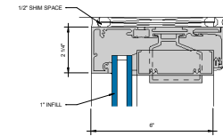
④ HEAD STANDARD RECEPTOR W/ OPTIONAL WEDGE GASKET 6" = 1'-0"
