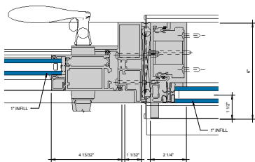
⑨ ALT. SSG DOOR JAMB @ LOCK STILE Ø = 1'-0"
