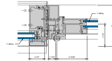
① DOOR JAMB @ HINGE STILE 6" = 1'-0"
