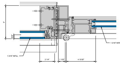
⑥ ALT. SSG DOOR JAMB @ HINGE STILE Ø = 1'-0"
