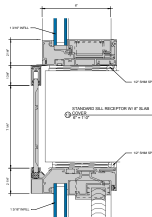
STANDARD HEAD RECEPTOR W/ ⑦ OPTIONAL BLIND POCKET 6" = 1'-0"
