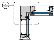
190 90° INSIDE CORNER 1 1/2" = 1'-0"
