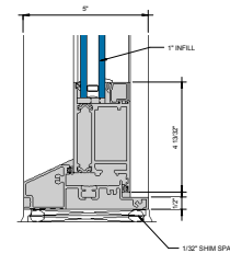
⑦ 2000T TERRACE DOOR SILL 6" = 1'-0"
