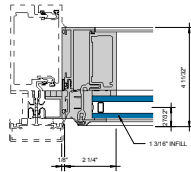
GLASSvent UT JAMB (LH) AT VERTICAL POCCOS Ø = 1-0"
