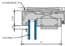
⑤ HEAD STANDARD RECEPTOR W/ REINFORCEMENT 6" = 1'-0"
