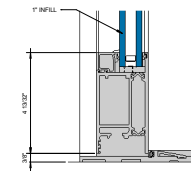
2000T TERRACE DOOR LOW PROFILE SILL ① 6" = 1'-0"
