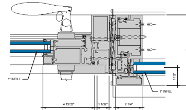
③ DOOR JAMB @ LOCK STILE Ø = 1'-0"
