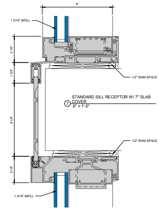
STANDARD HEAD RECEPTOR W/ ④ OPTIONAL WEDGE GASKET 6" = 1'-0"
