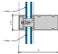
⑥ HORIZONTAL 6" = 1'-0"
