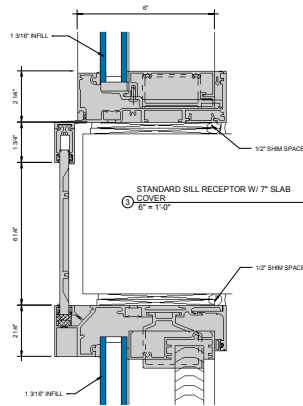
STANDARD HEAD RECEPTOR W/ ② OPTIONAL BLIND POCKET 6" = 1'-0"
