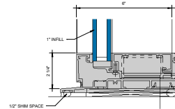
③ SILL PUNCHED OPENING RECEPTOR 6" = 1'-0"
