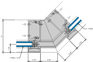
⑤ 135° OUTSIDE CORNER G = 1'-0"
