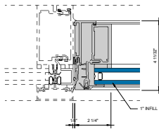
GLASSvent UT JAMB (LH) AT VERTICAL RECEPTOR ① 6" = 1'-0"
