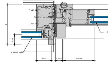
⑦ ALTERNATE SSG DOOR JAMB @ HINGE STILE 6" = 1'-0"
