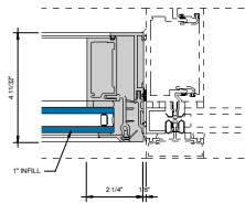
GLASSvent UT JAMB (RH) AT VERTICAL RECEPTOR ① 6" = 1'-0"
