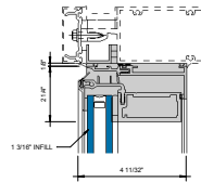
GLASSvent UT HEAD AT HORIZONTAL POCCOS Ø = 1-0"
