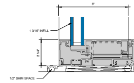
⑧ SILL STANDARD RECEPTOR 6" = 1'-0"
