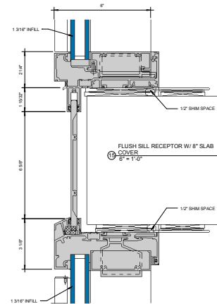
⑨ FLUSH HEAD RECEPTOR W/ OPTIONAL STRAP ANCHOR 6" x 1'-0"
