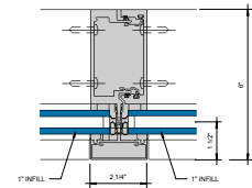
④ VERTICAL MULLION 6" = 1'-0"
