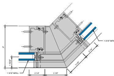
⑥ 135° OUTSIDE CORNER (SSG) G = 1'-0"
