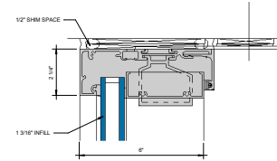
③ HEAD STANDARD RECEPTOR W/ OPTIONAL STRAP ANCHOR 6" = 1'-0"
