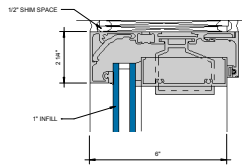
⑤ HEAD STANDARD RECEPTOR W/ REINFORCEMENT 6" = 1'-0"
