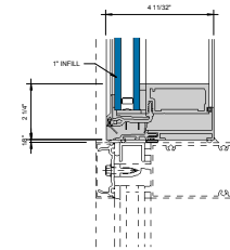
GLASSvent UT SILL AT HORIZONTAL RECEPTOR ① 6" = 1'-0"
