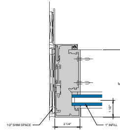
③ JAMB RECEPTOR AND STRAP ANCHOR 6" = 1'-0"
