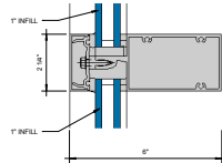
② HORIZONTAL 6" = 1'-0"
