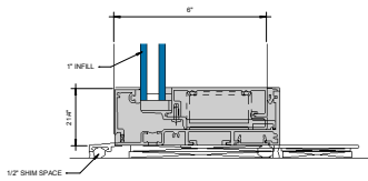
SILL STANDARD RECEPTOR W/ ⑨ OPTIONAL STRAP ANCHOR 6" x 1-1/2"
