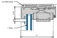
① HEAD STANDARD RECEPTOR 6" x 1-1/2"
