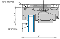
① HEAD PUNCHED OPENING RECEPTOR 6" = 1'-0"
