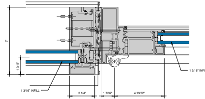
② DOOR JAMB @ HINGE STILE Ø = 1'-0"
