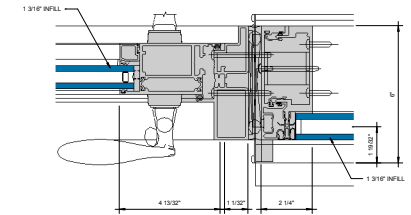
8 ALTERNATE. SSG DOOR JAMB @ LOCK STILE 6" = 1'-0"
