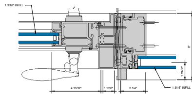
6 ALTERNATE. SSG DOOR JAMB @ LOCK STILE 6" = 1'-0"
