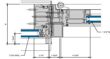
7 ALTERNATE. SSG DOOR JAMB @ HINGE STILE 6" = 1'-0"
