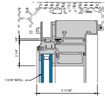
GLASSvent UT HEAD AT HEAD RECEPTOR POCCOS Ø = 1-0"
