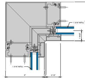
③ 90° INSIDE CORNER G = 1'-0"
