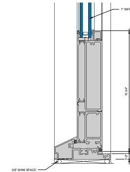
⑧ 2000T TERRACE DOOR 10" TALL SILL 6" = 1'-0"
