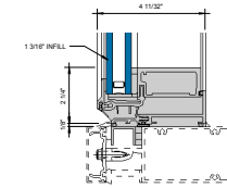
GLASSvent UT SILL AT HORIZONTAL POCCOS Ø = 1-0"
