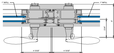
⑨ MEETING STILES 6" = 1'-0"
