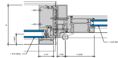
⑫ DOOR JAMB @ HINGE STILE 6" = 1'-0"
