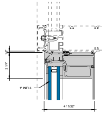
GLASSvent UT HEAD AT HORIZONTAL RECEPTOR ① 6" = 1'-0"
