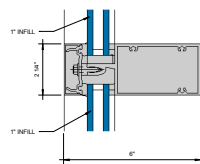
⑥ HORIZONTAL 6" x 1-1/2"
