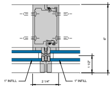
⑤ ALT. SSG VERTICAL MULLION Ø = 1'-0"
