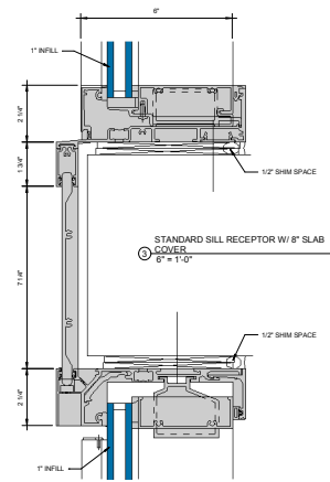
STANDARD HEAD RECEPTOR W/ REINFORCEMENT ④ 6" x 11-0"
