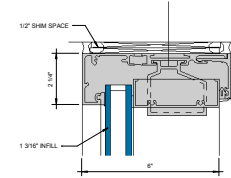
④ HEAD STANDARD RECEPTOR W/ OPTIONAL WEDGE GASKET 6" = 1'-0"
