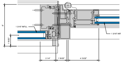
5 ALTERNATE. SSG DOOR JAMB @ HINGE STILE 6" = 1'-0"
