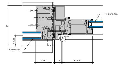
⑧ ALT. SSG DOOR JAMB @ HINGE STILE Ø = 1'-0"
