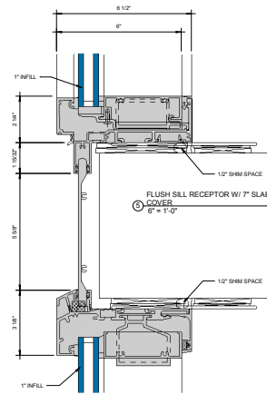
FLUSH HEAD RECEPTOR W/ OPTIONAL ① STRAP ANCHOR ② 6" x 1"-0"
