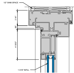
⑥ 2000T TERRACE DOOR HEADER W/ PUNCHED OPENING RECEPTOR 6" = 1'-0"
