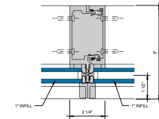
④ ALT. SSG VERTICAL MULLION 6" = 1'-0"
