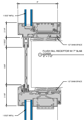
② FLUSH HEAD RECEPTOR 6" = 1'-0"
