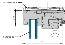
② HEAD STANDARD RECEPTOR W/ OPTIONAL BLIND POCKET 6" = 1'-0"
