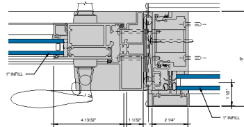
② DOOR JAMB @ LOCK STILE 6" = 1'-0"
