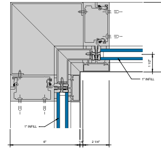
③ 90° INSIDE CORNER G = 1'-0"
