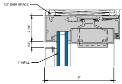
TRANSOM HEAD W/ PUNCHED OPENING RECEPTOR ① 6" = 1'-0"
