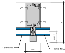
⑤ ALT. SSG VERTICAL MULLION Ø = 1'-0"
