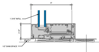
⑨ SILL STANDARD RECEPTOR W/ OPTIONAL STRAP ANCHOR 6" = 1'-0"
