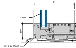
③ SILL W/ PUNCHED OPENING RECEPTOR 6" = 1'-0"
