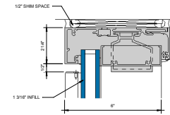
④ HEAD STANDARD RECEPTOR W/ OPTIONAL WEDGE GASKET 6" = 1'-0"
