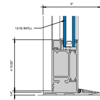
⑧ 2000T TERRACE DOOR LOW PROFILE SILL 6" = 1'-0"
