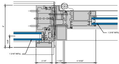
1 DOOR JAMB @ HINGE STILE 6" = 1'-0"
