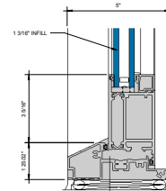
⑦ 2000T TERRACE DOOR SILL 6" = 1'-0"
