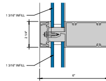
⑥ HORIZONTAL 6" = 1'-0"
