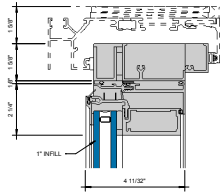
GLASSvent UT HEAD AT HEAD RECEPTOR POICOS ① 6" = 1'-0"
