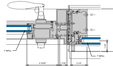
⑦ ALT. SSG DOOR JAMB @ LOCK STILE Ø = 1'-0"
