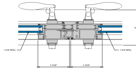
⑩ 2000T DOOR MEETING STILES Ø = 1'-0"
