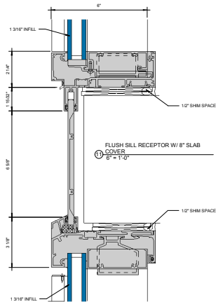
⑦ FLUSH SILL RECEPTOR 6" x 1'-0"
