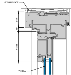
2000T TERRACE DOOR HEADER W/ PUNCHED OPENING RECEPTOR ① 6" = 1'-0"
