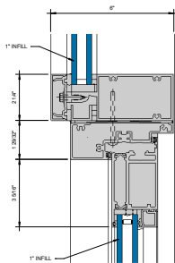
2000T TERRACE DOOR HEADER @ HORIZONTAL ⑤ 6" = 1'-0"
