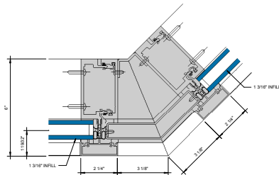
⑤ 135° OUTSIDE CORNER G = 1'-0"
