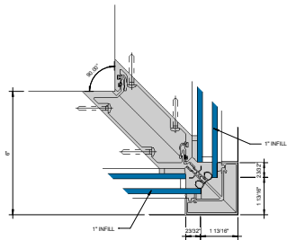
① 90° OUTSIDE CORNER G = 1'-0"
