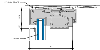
HEAD STANDARD RECEPTOR W/ ③ OPTIONAL STRAP ANCHOR 6" x 1-1/2"
