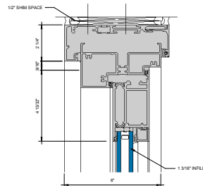
⑥ 2000T TERRACE DOOR HEADER W/ PUNCHED OPENING RECEPTOR 6" = 1'-0"
