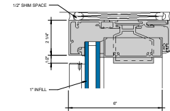
HEAD STANDARD RECEPTOR W/ ④ OPTIONAL WEDGE GASKET 6" x 1-1/2"
