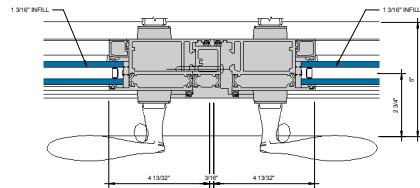
9 MEETING STILES 6" = 1'-0"
