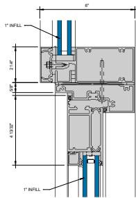
2000T TERRACE DOOR HEADER @ HORIZONTAL ① 6" = 1'-0"
