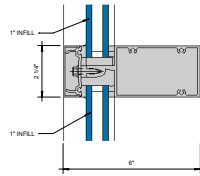
② HORIZONTAL 6" = 1'-0"
