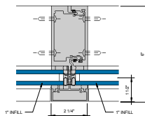
⑩ VERTICAL MULLION 6" = 1'-0"
