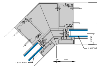
⑦ 135° INSIDE CORNER G = 1'-0"
