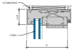
① HEAD STANDARD RECEPTOR 6" = 1'-0"
