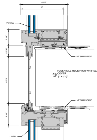
FLUSH HEAD RECEPTOR W/ OPTIONAL ① STRAP ANCHOR ② 6" x 1"-0"
