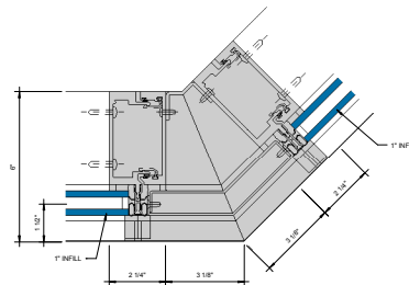
⑥ 135° OUTSIDE CORNER (SSG) G = 1'-0"
