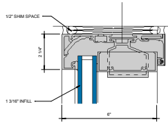
⑤ HEAD STANDARD RECEPTOR W/ REINFORCEMENT 6" = 1'-0"
