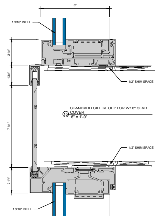
STANDARD HEAD RECEPTOR W/ ⑧ OPTIONAL STRAP ANCHOR 6" = 1'-0"
