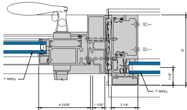
① DOOR JAMB @ LOCK STILE Ø = 1'-0"
