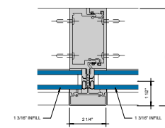
⑪ VERTICAL MULLION 6" = 1'-0"
