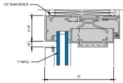
TRANSOM HEAD W/ PUNCHED OPENING RECEPTOR ① 6" = 1'-0"
