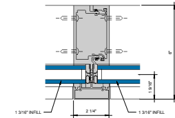
④ VERTICAL MULLION h = 1'-0"
