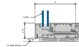
⑧ SILL STANDARD RECEPTOR 6" = 1'-0"
