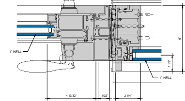
⑧ ALTERNATE SSG DOOR JAMB @ LOCK STILE 6" = 1'-0"
