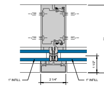
① VERTICAL MULLION 6" = 1'-0"
