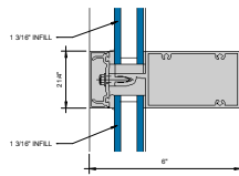
⑥ HORIZONTAL 6" = 1'-0"
