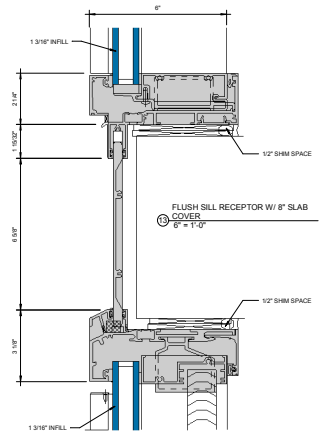
⑧ FLUSH HEAD RECEPTOR W/ OPTIONAL BLIND POCKET 6" x 1'-0"
