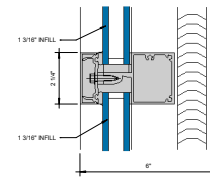
⑦ HORIZONTAL BLIND APPLICATION 6" = 1'-0"
