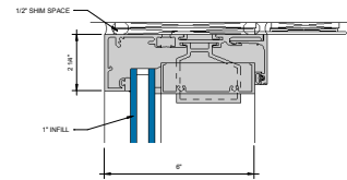
③ HEAD STANDARD RECEPTOR W/ OPTIONAL STRAP ANCHOR 6" = 1'-0"
