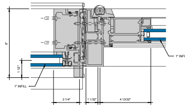
⑤ ALTERNATE SSG DOOR JAMB @ HINGE STILE 6" = 1'-0"
